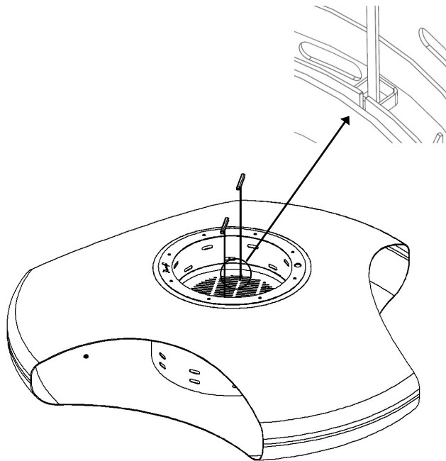
Figure 8 – Handle fitting
