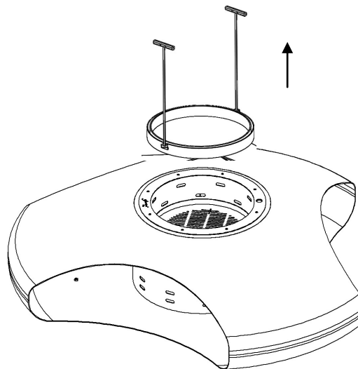
Figure 9 – Ashtray removal
